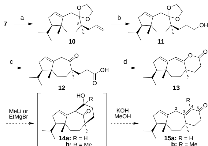
Scheme 2. Synthesis of dienol lactone 13 and attempted Turner–Fujimoto reactions. a) Ethylene glycol, TsOH, benzene, reflux, [-\text{H}_2\text{O}] , 36 h, 89%; b) 1) 9-BBN, THF, 0^\circ\text{C} \rightarrow \text{RT} , 3.5 h; 2) NaOH (aqueous, 3 N), \text{H}_2\text{O}_2 (aqueous, 30%), room temperature, 1.5 h, 98%; c) \text{CrO}_3 , \text{H}_2\text{SO}_4 , acetone, room temperature, 2 h, 62%; d) NaOAc, \text{Ac}_2\text{O} , 140^\circ\text{C} , 80 min, 59%. TsOH = p -toluene sulfonic acid, 9-BBN = 9-borabicyclo[3.3.1]nonane.
